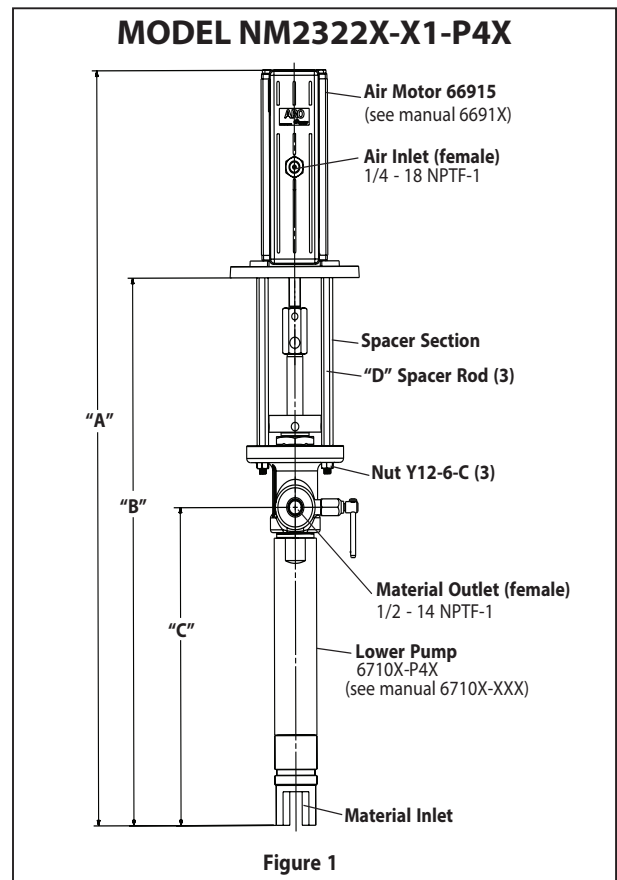
NOTE: Dimensions are shown in inches and (mm) and are supplied for reference only.
